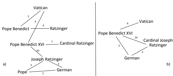
FIGURE 1: a) Example graph after creating contexts. b) After merging all direct co-references.
